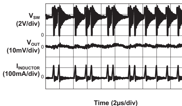
Step-Down Converter Output Ripple ( V_{SYSOUT} = 5.0V , V_{OUT} = 3.3V , I_{LOAD} = 10mA ; C_{SYSOUT} = C_{OUT} = 22\mu F , L = 2.2\mu H )
