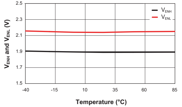
Switch V_{ENH} and V_{ENL} vs. Temperature ( V_{IN} = 5.0V ; R_{SET} = 11.3K\Omega )
